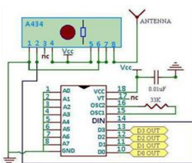
Figure 6: Circuit Diagram of RF Receiver with HT12D decoder IC
