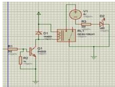
Figure 8: Transistor operated relay circuit
