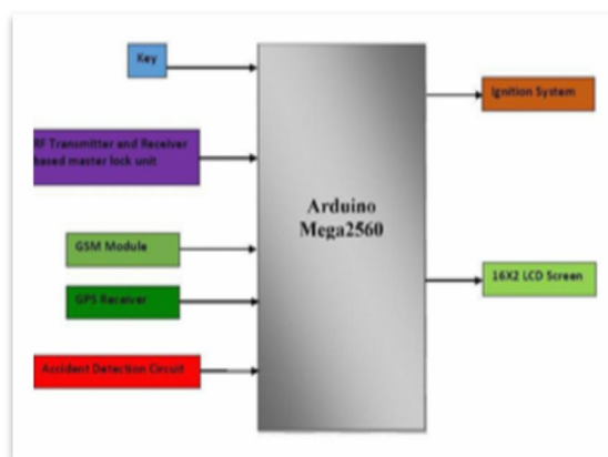
Figure 1: Proposed telematics module block diagram\
