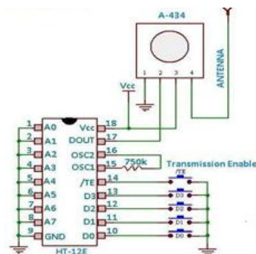
Figure 5: Circuit Diagram of RF Transmitter with HT12E encode IC
